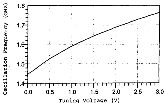
Fig.4. Tuning characteristic of the quadrature VCO.
