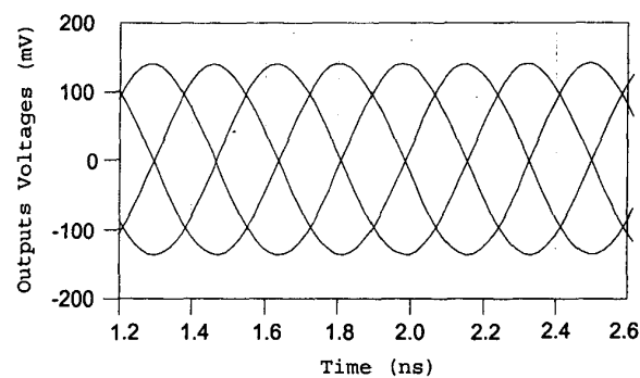
Fig.6. Output Quadrature Waveforms of the VCO.
