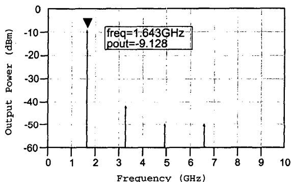
Fig.5. Simulated output spectrum of the VCO.
